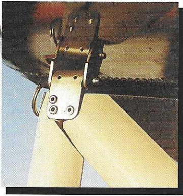
Reduce drag with these jury strut fairings.
